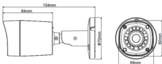
Dimensions (mm)
