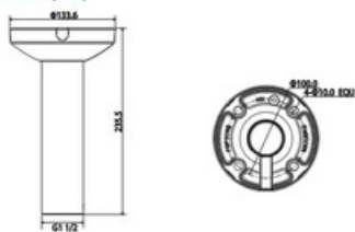
Dimensions (mm)
