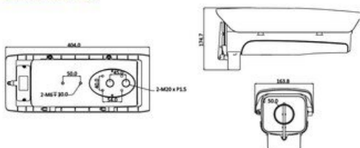
Dimensions (mm)
